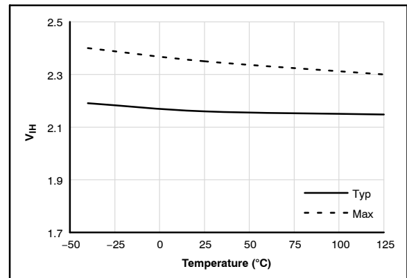
Figure 25. Logic HIGH Input Voltage vs. Temperature
