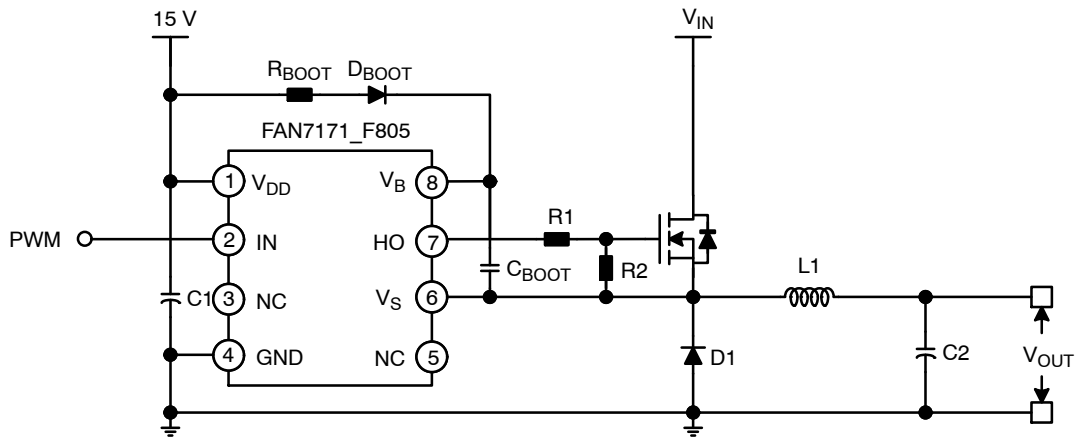
Figure 1. Typical Application
