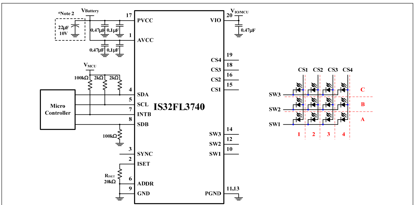
Figure 1 Typical Application Circuit (3×4)
