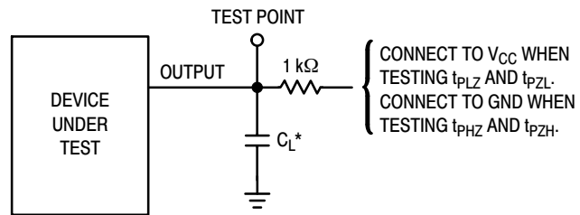
Figure 8. Test Circuit
