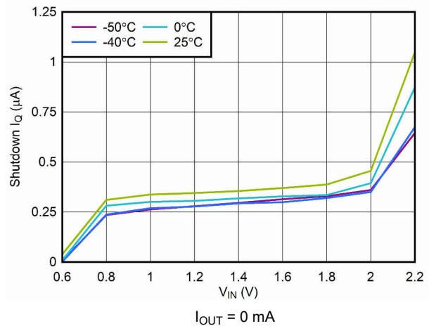
Figure 6-8. V_{\text{IN}} Shutdown I_{\text{Q}} vs V_{\text{IN}}
