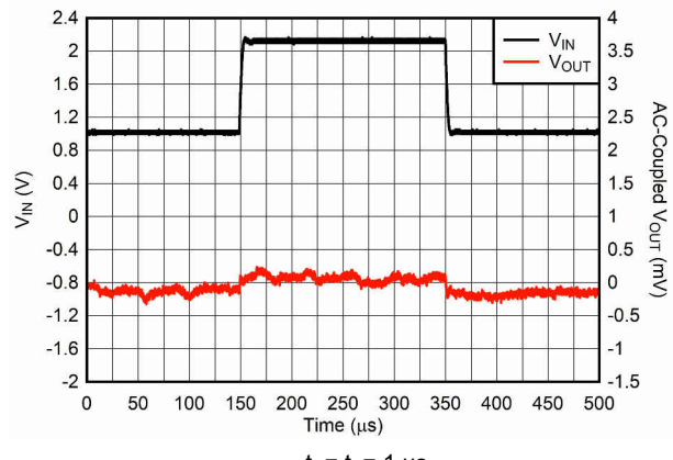
Figure 6-18. Line Transient From 1 V to 2.2 V
