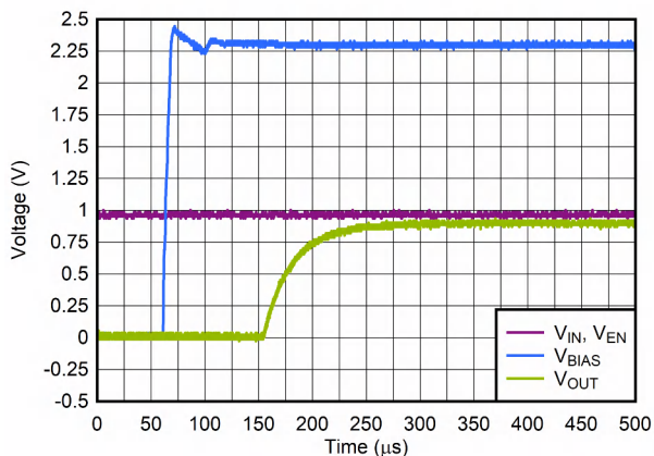
Figure 6-17. Start-Up With V_{\text{IN}} and V_{\text{EN}} Before V_{\text{BIAS}}
