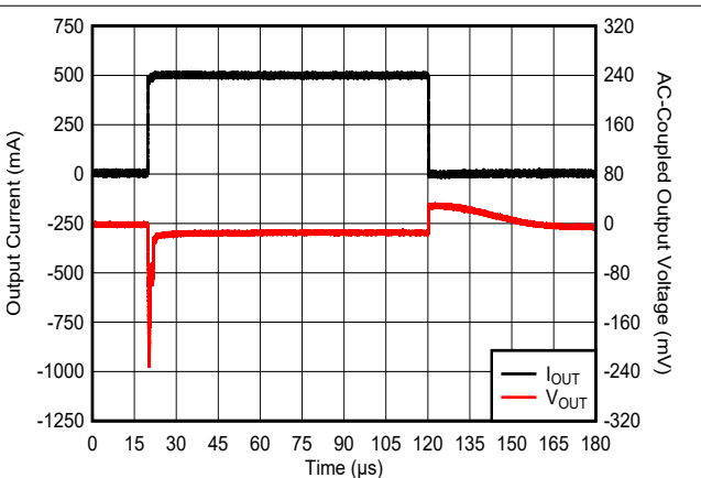
V_{EN} = V_{IN} , t_r = t_f = 200\text{ ns}
